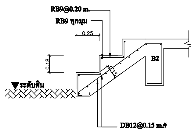
ST-1 SCALE 1:25
