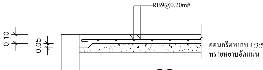
GS SCALE 1:25
