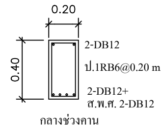
B2 SCALE 1:25
