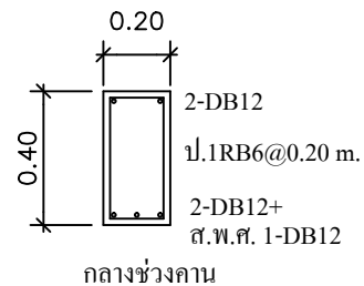
B1 SCALE 1:25
