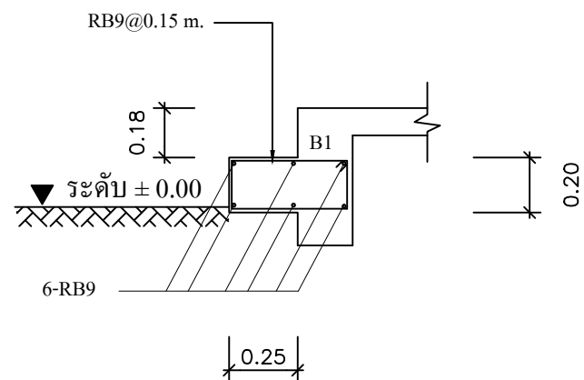
ST-1, ST-2 SCALE 1:25
