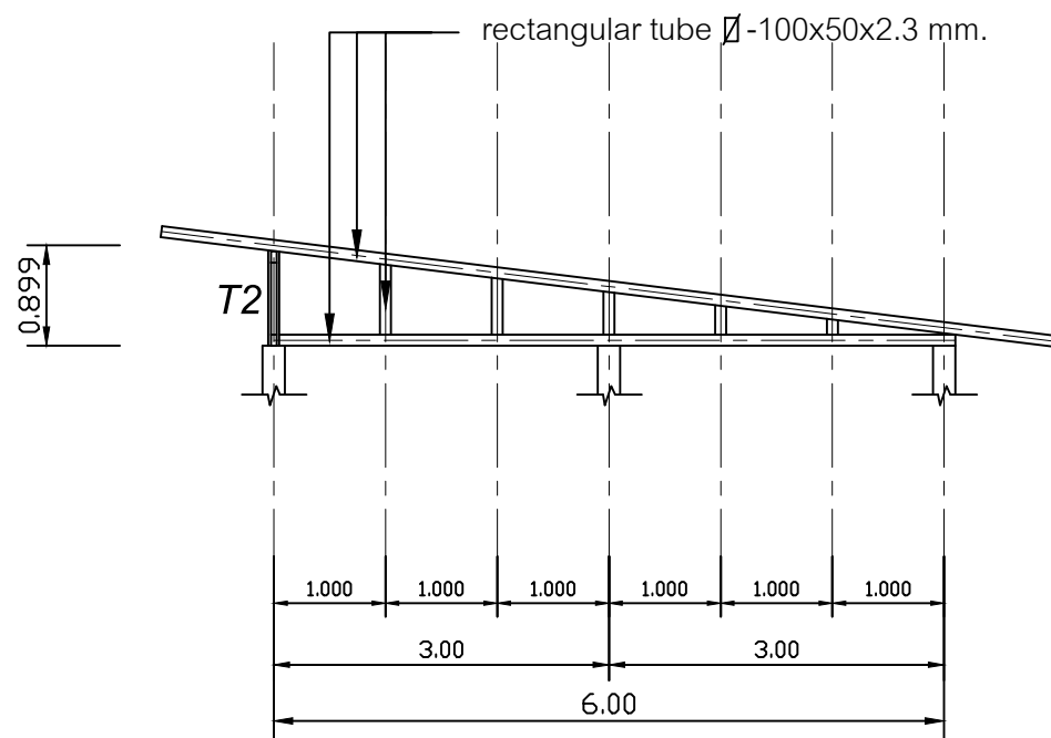
TRUSS T1
