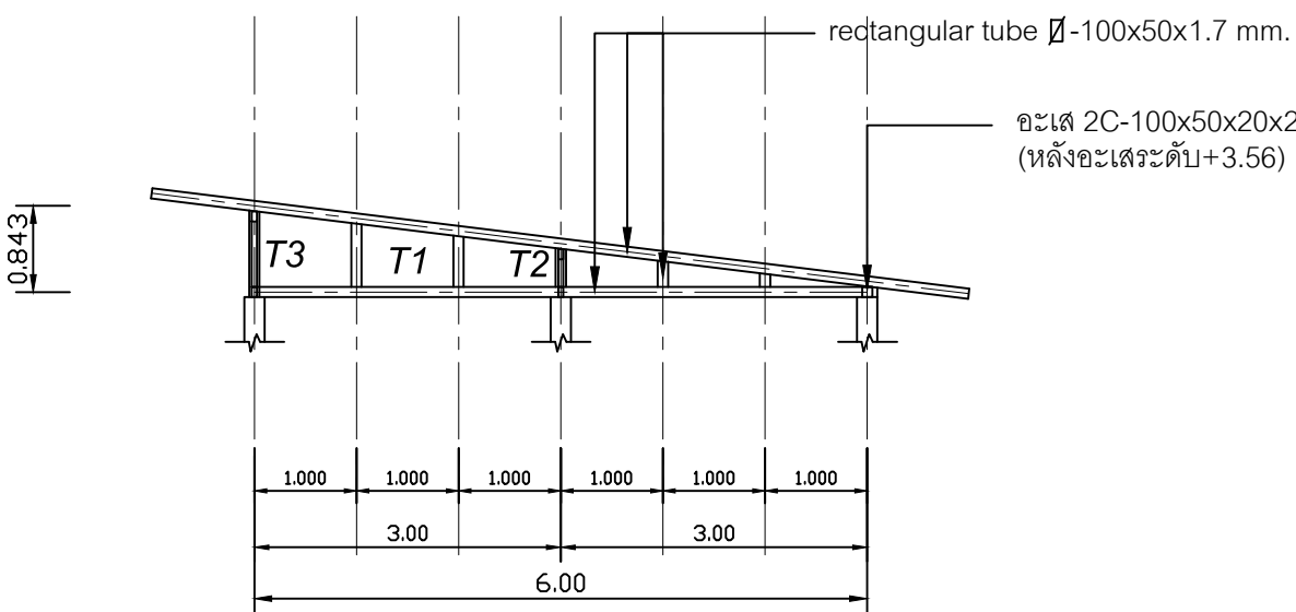
TRUSS T1
