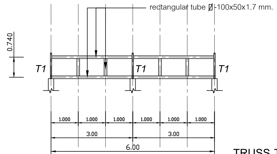
TRUSS T3
